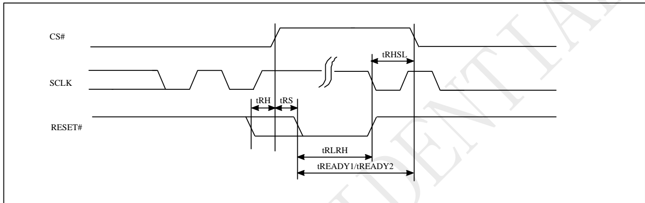
Figure 10-58 RESET Timing
