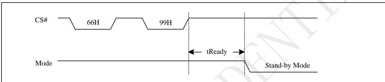
Figure 10-55a Reset Sequence
