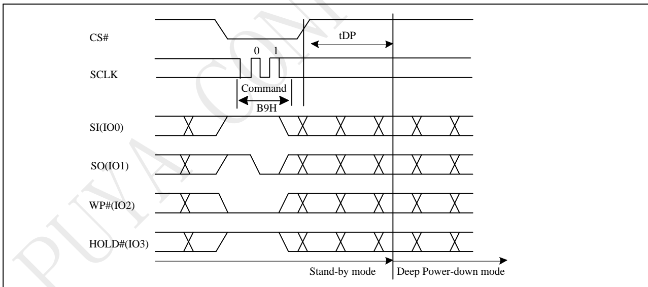
Figure 10-40a Deep Power-down (DP) Sequence (QPI)
