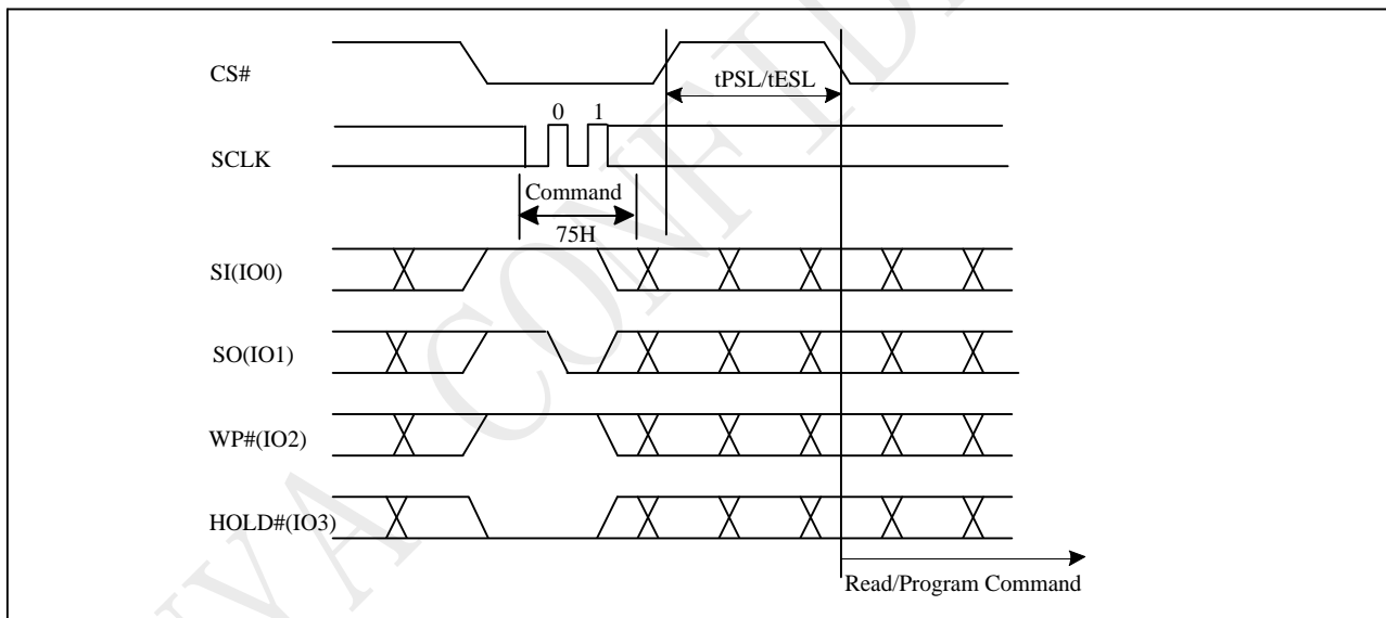
Figure 10-47a Suspend to Read/Program Latency(QPI)
